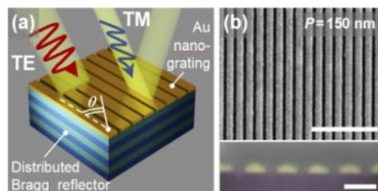
Fig. 3. Polarisation-sensitive hybrid metal-dielectric mirror. (a) Schematics of the hybrid mirror interacting with normally incident linearly polarised light. Angle \theta shows the azimuth of incident polarisation. (b) SEM images of Au wire-grid nanogratings with periods of 150 \text{ nm} fabricated on top of a conventional distributed Bragg reflector. The scale bar is 150 \text{ nm} .
