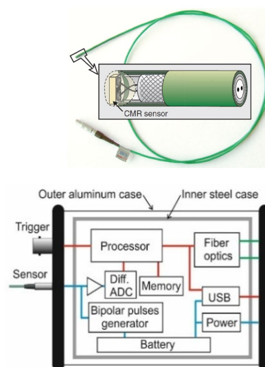
Fig. 7. (Top) Cross-section of CMR sensor. (Bottom) Block diagram of the measure module.
