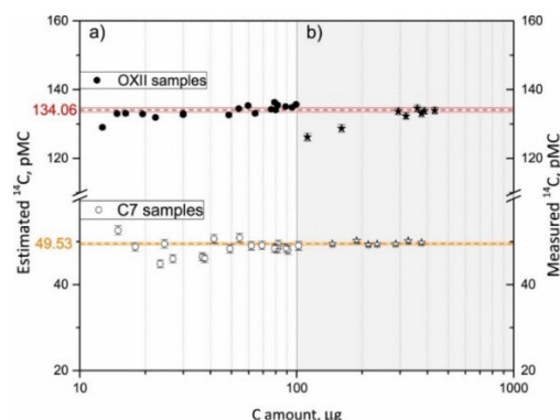
Fig. 7. Estimated and measured pMC values of samples with known pMC: (a) prepared and measured by dilution method (carbon amount 15\text{--}100\text{ }\mu\text{g} ) and (b) measured ^{14}\text{C} values of the samples prepared using the conventional method (carbon amount 100\text{--}500\text{ }\mu\text{g} ). The red line shows the nominal pMC values for investigated samples.
