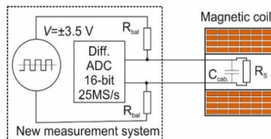
Fig. 6. Block diagram of a measurement system.
